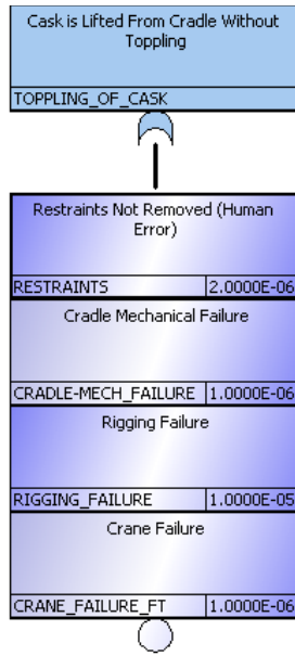
Figure 10-20. Fault tree 5.1, cask is lifted from cradle without toppling.
