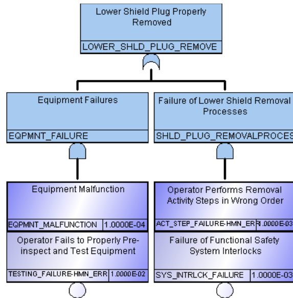
Figure 10-30. Fault tree 6.3, lower shield plug properly removed.
