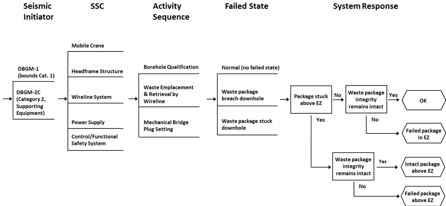
Figure 12-4. Example summary seismic event sequence diagram for supporting equipment (wireline and borehole event hazard categories)
