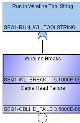
Figure 10-2. Fault tree 1.2, run in wireline tool string.
