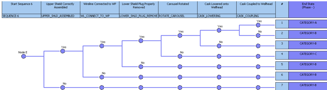
Figure 9-5. Event tree for Sequence 6, configure waste package, wellhead and wireline for emplacement.
