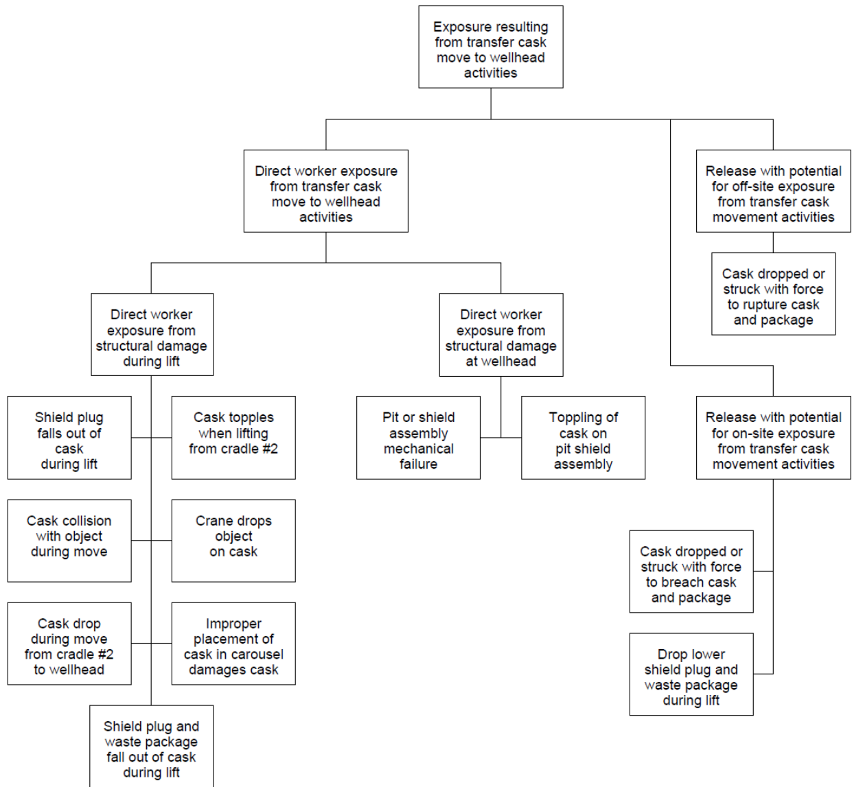
Figure 8-4. MLD detail for transfer cask move to the wellhead events.
