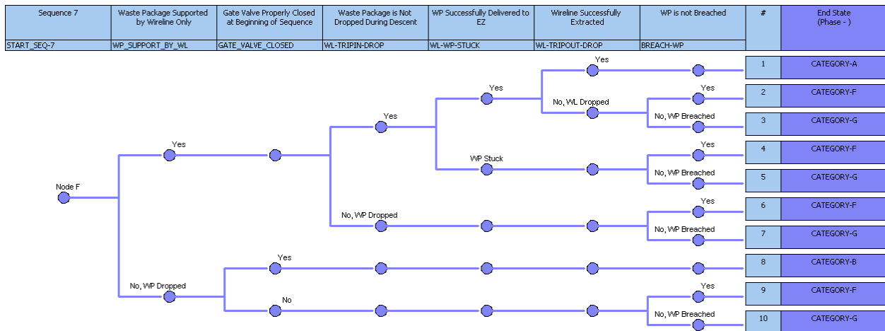
Figure 9-6. Event tree for Sequence 7, waste package emplacement, release, and wireline retrieval.
