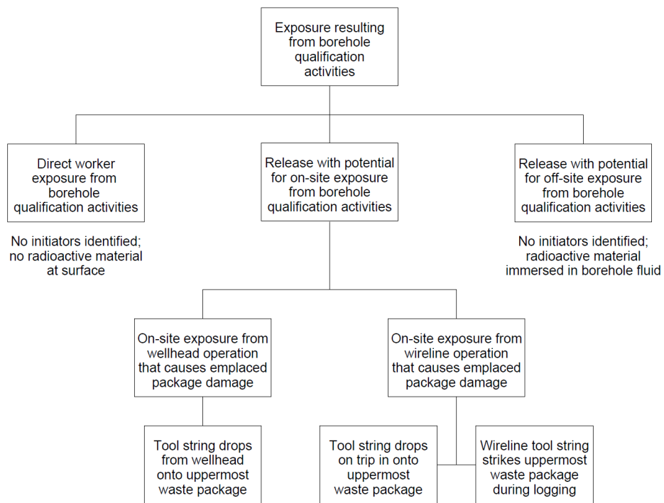
Figure 8-7. MLD detail for borehole qualification events.
