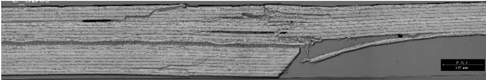
Cross-Section of BVID at a Skin-to-Flange
