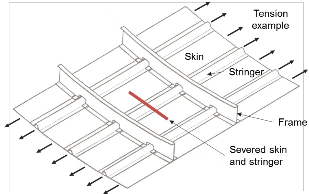
Fuselage Skin-Stringer Panel with Notch
