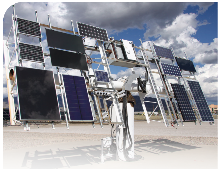
The primary testing tracker, with multiple PV modules, at Sandia's Photovoltaic Systems Evaluation Laboratory
