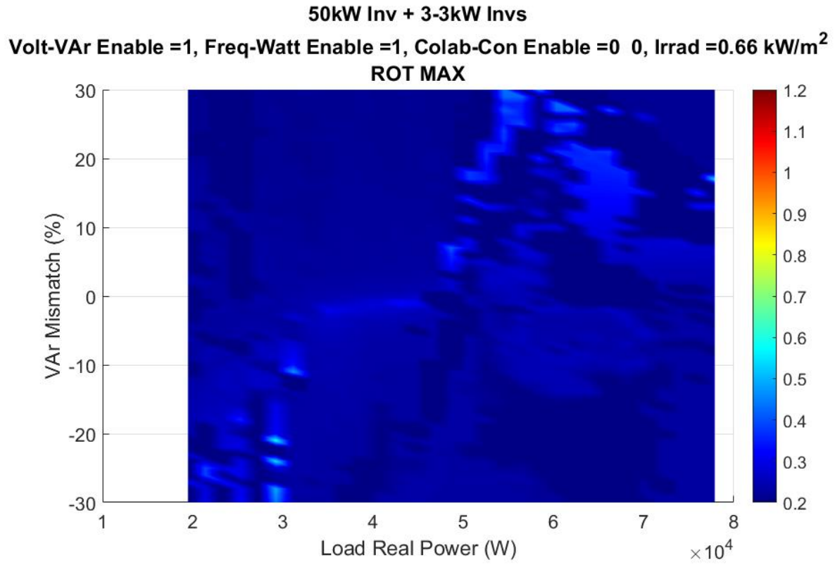
Figure 50. X-y plane view of Figure 49.
