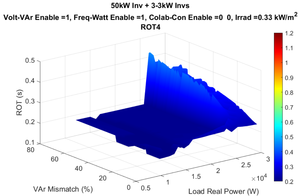
Figure 43. ROTs vs. var mismatch and load real power power, 33% irradiance.
