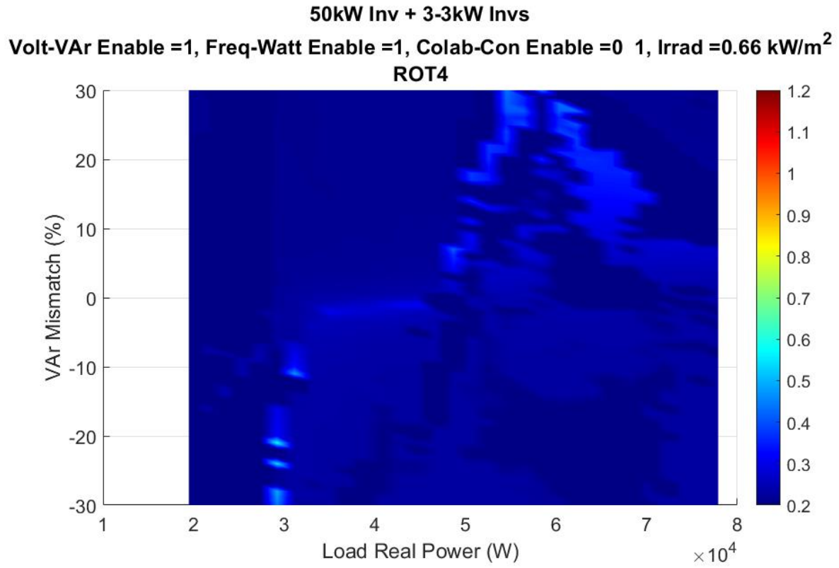
Figure 60. X-y plane view of Figure 59.
