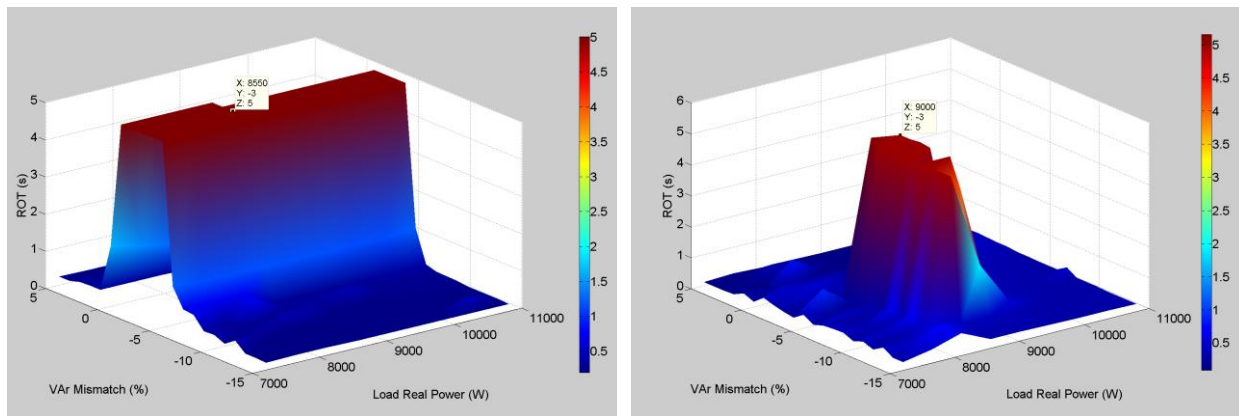
Figure 9. ROTs vs. P and Q mismatch for 100% irradiance. Left: no GSFs. Right: GSFs active.
