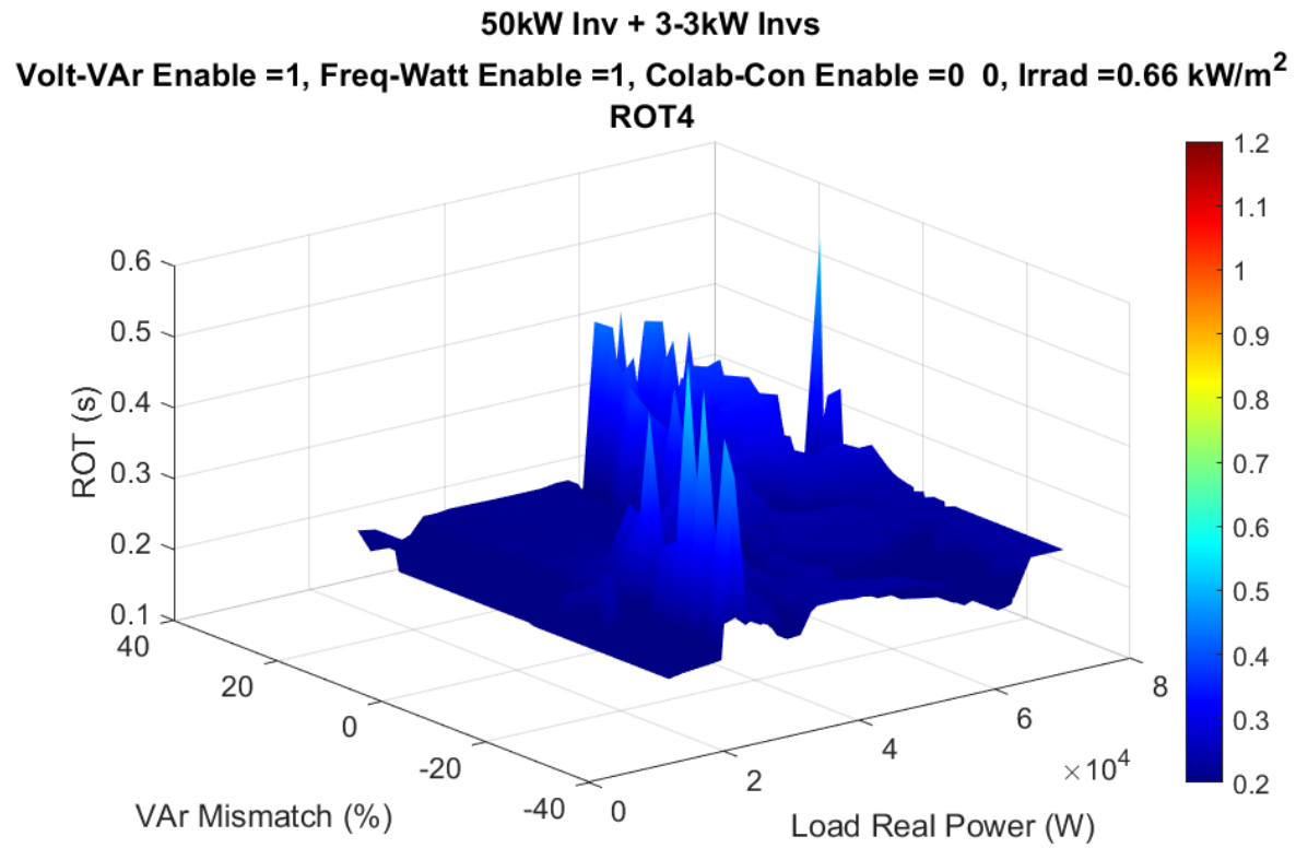
Figure 47. ROTs vs. var mismatch and load real power, 66% irradiance.
