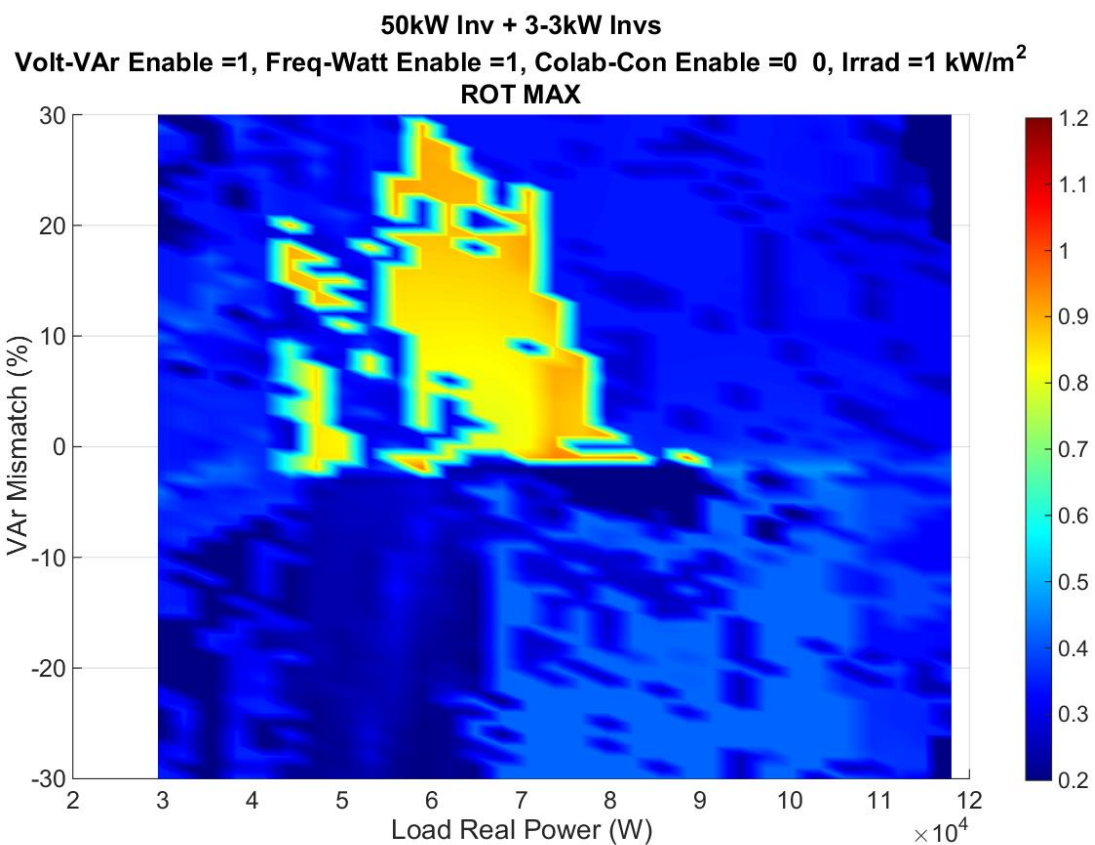
Figure 78. X-y plane view of Figure 77.
