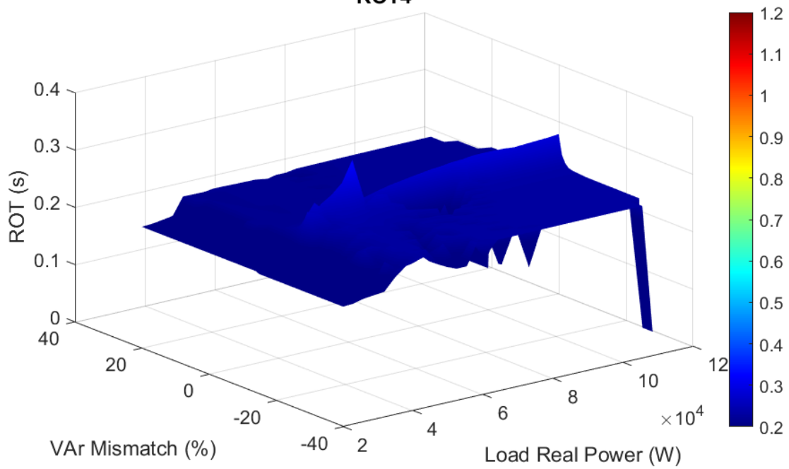
Figure 63. ROTs vs. var mismatch and load real power, 100% irradiance.
