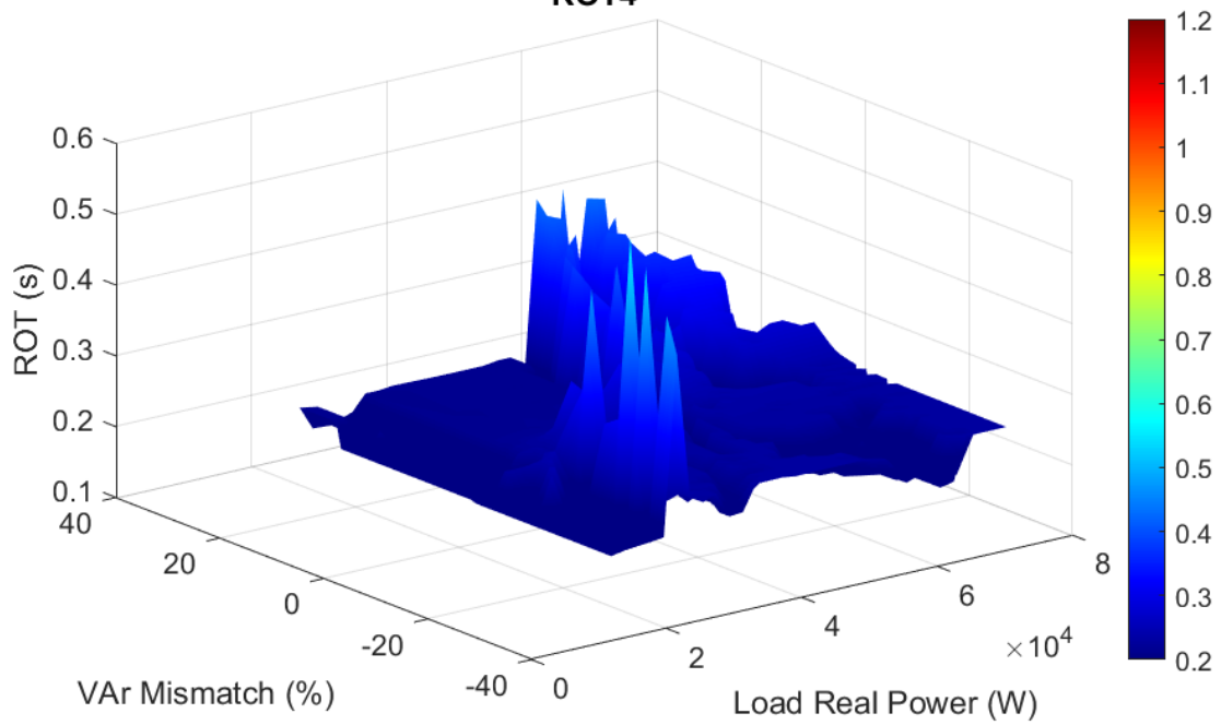
Figure 59. ROTs vs. var mismatch and load real power, 66% irradiance.
