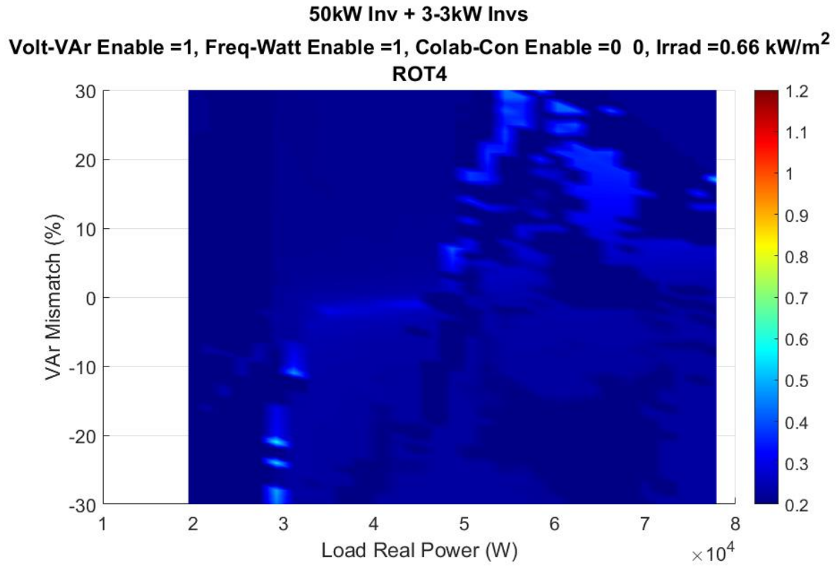
Figure 48. X-y plane view of Figure 47.
