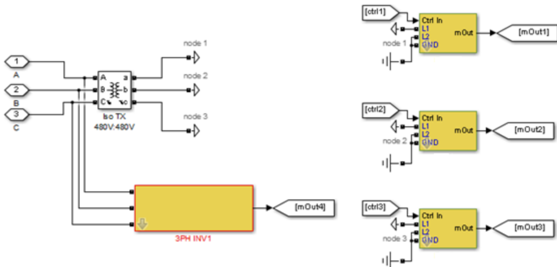
Figure 13. This figure shows the contents of the green inverter block in Figure 12. The three units of Inverter A are isolated by a 480V:480V Yg-Yg tx and connected line to ground (wye). Inverter B is connected directly to the 480V bus.
