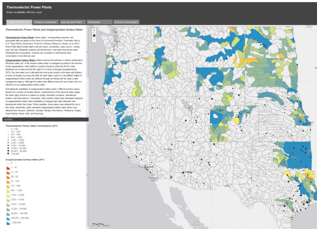
Figure 3. Map showing estimated water consumption for power plants in the project area. The map is reproduced from the project website. This data and other power plant water use information can be accessed on the project website.
