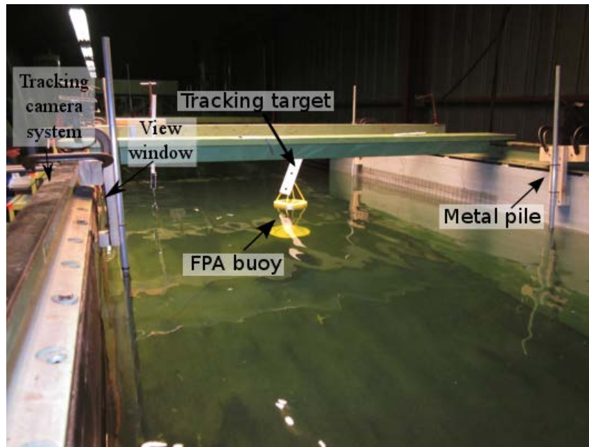
Figure 2. Locked FPA wave tank test and instrumentation setup. Photo by Ye Li, NREL 20118
