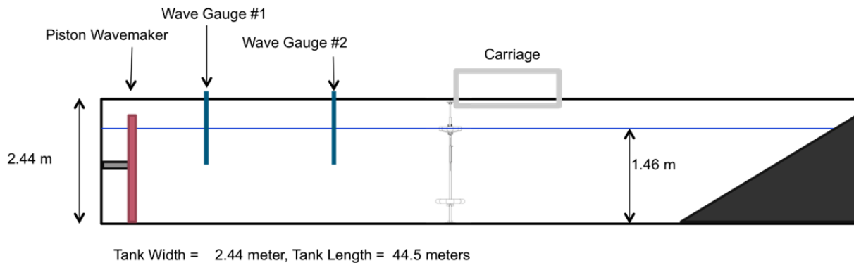
Figure 7. Schematic of the wave tank at the Scripps Institution of Oceanography at the University of California at San Diego
