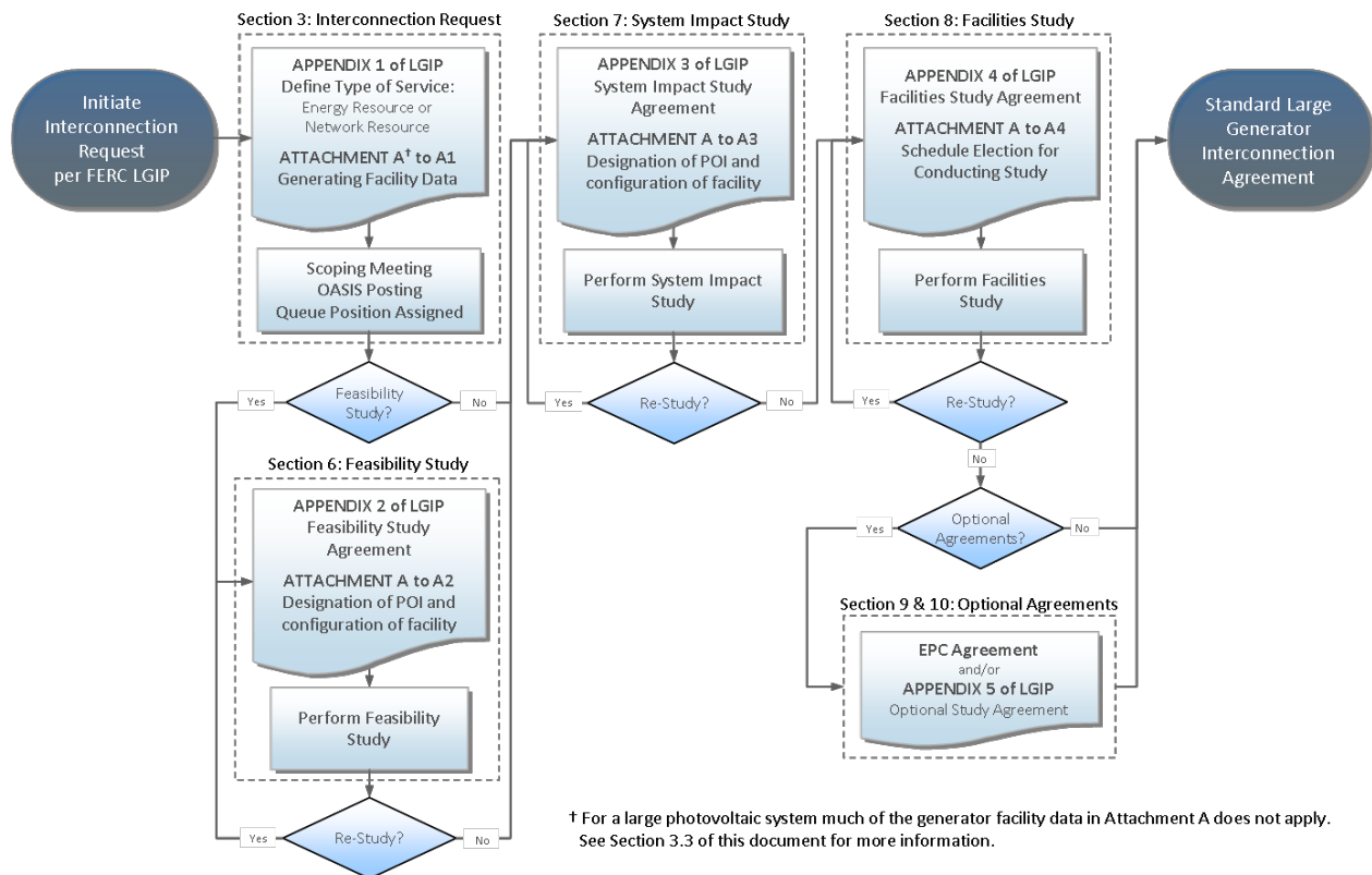
Figure 8. FERC Standard Large Generator Interconnection Procedure flowchart.
