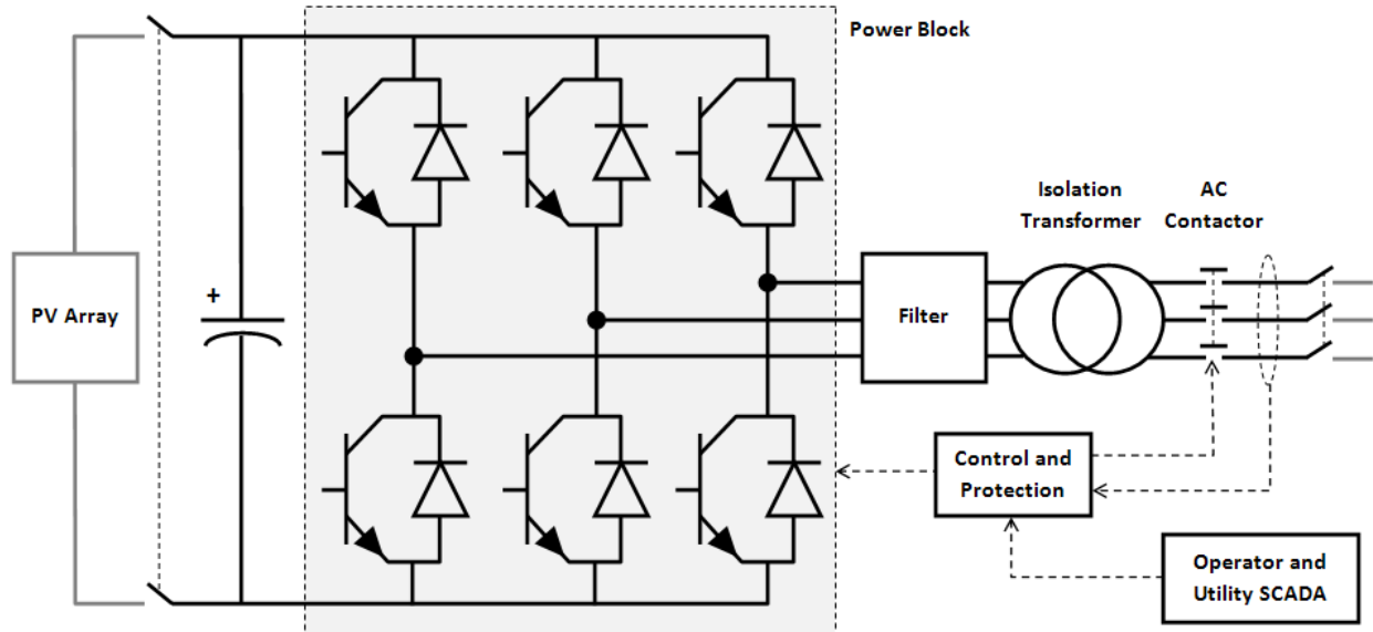
Figure 7. Example of PV inverter topology.
