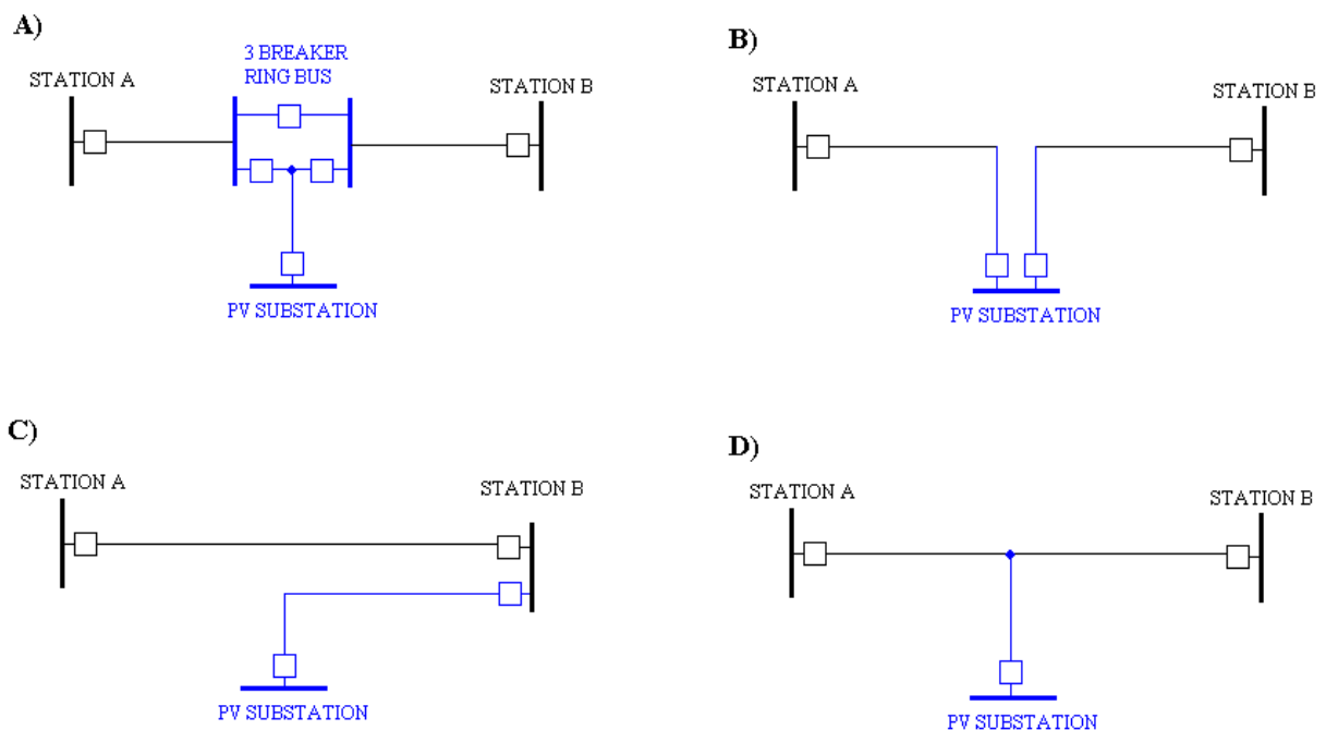
Figure 12. Examples of possible options for generator facility interconnection.
