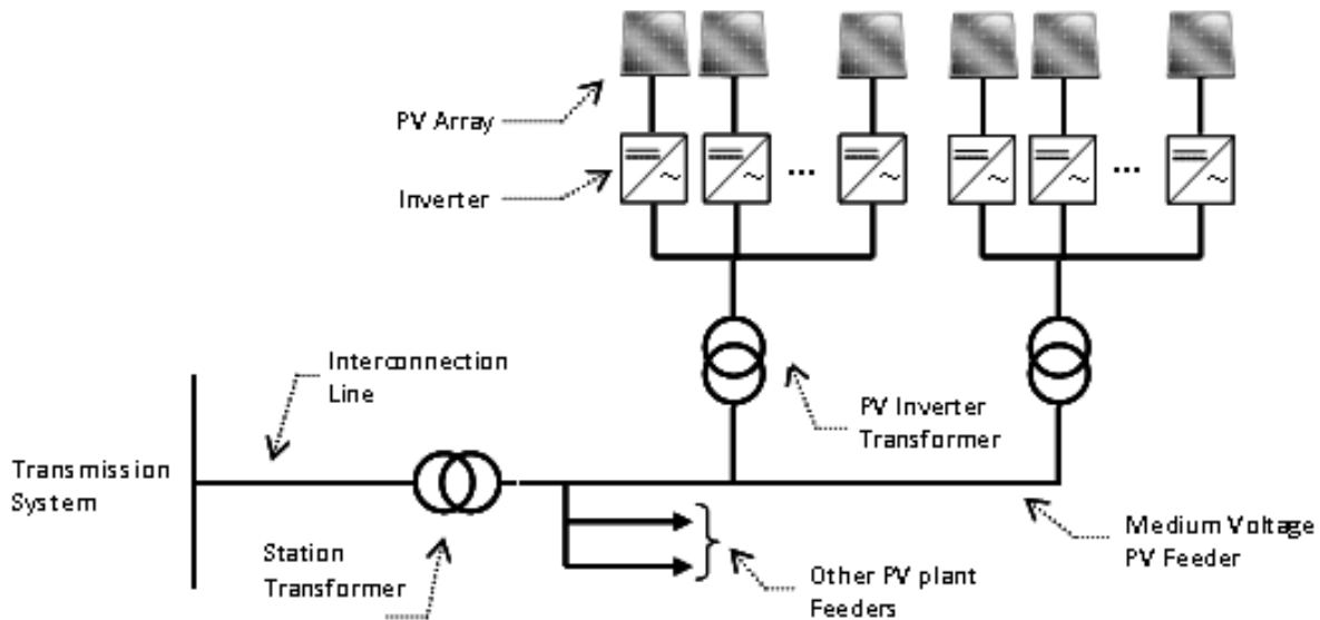
Figure 6. PV plant topology.
