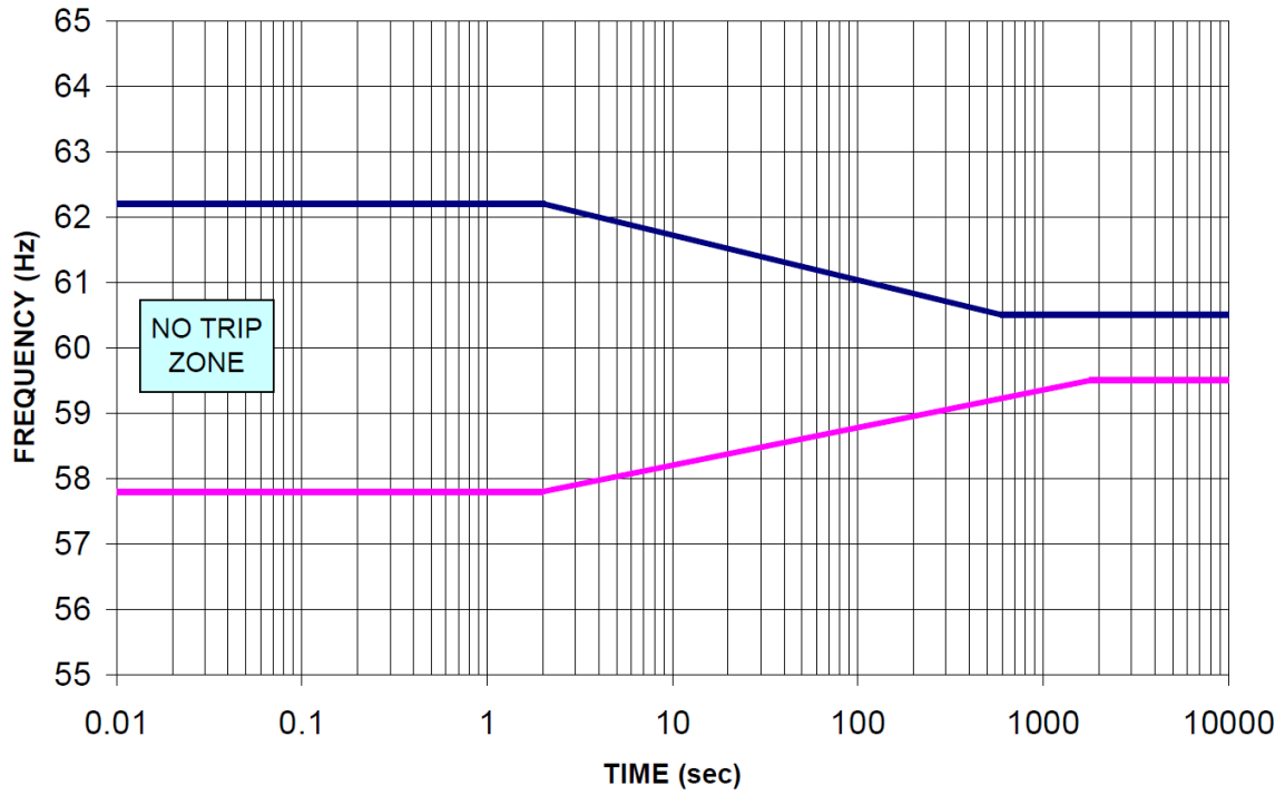
Figure 11. NERC PRC-024 and WECC frequency ride-through curves.
