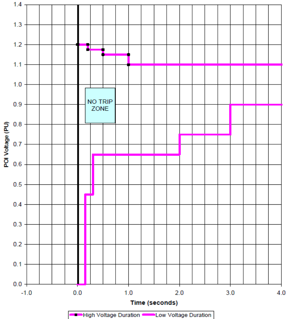
Figure 10. Proposed NERC PRC-024-1 VRT curve.
