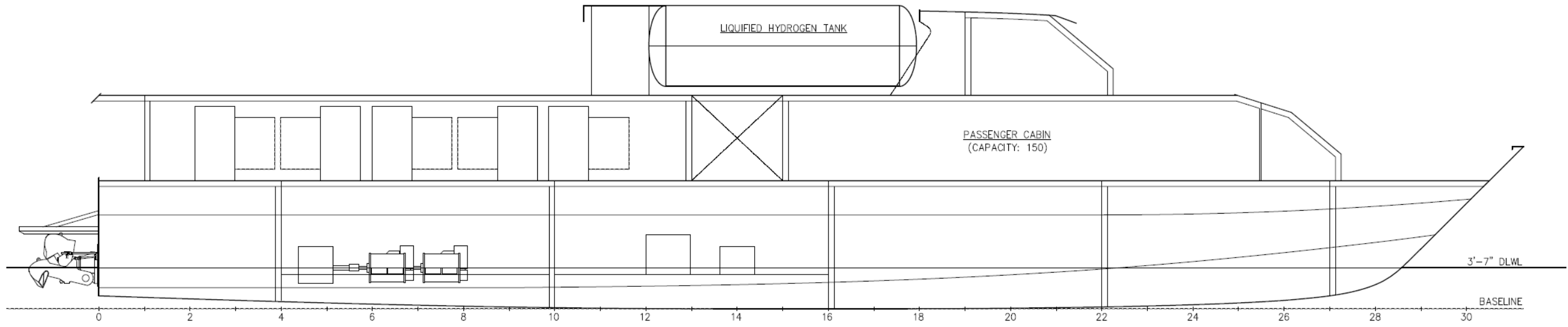
INBOARD PROFILE
