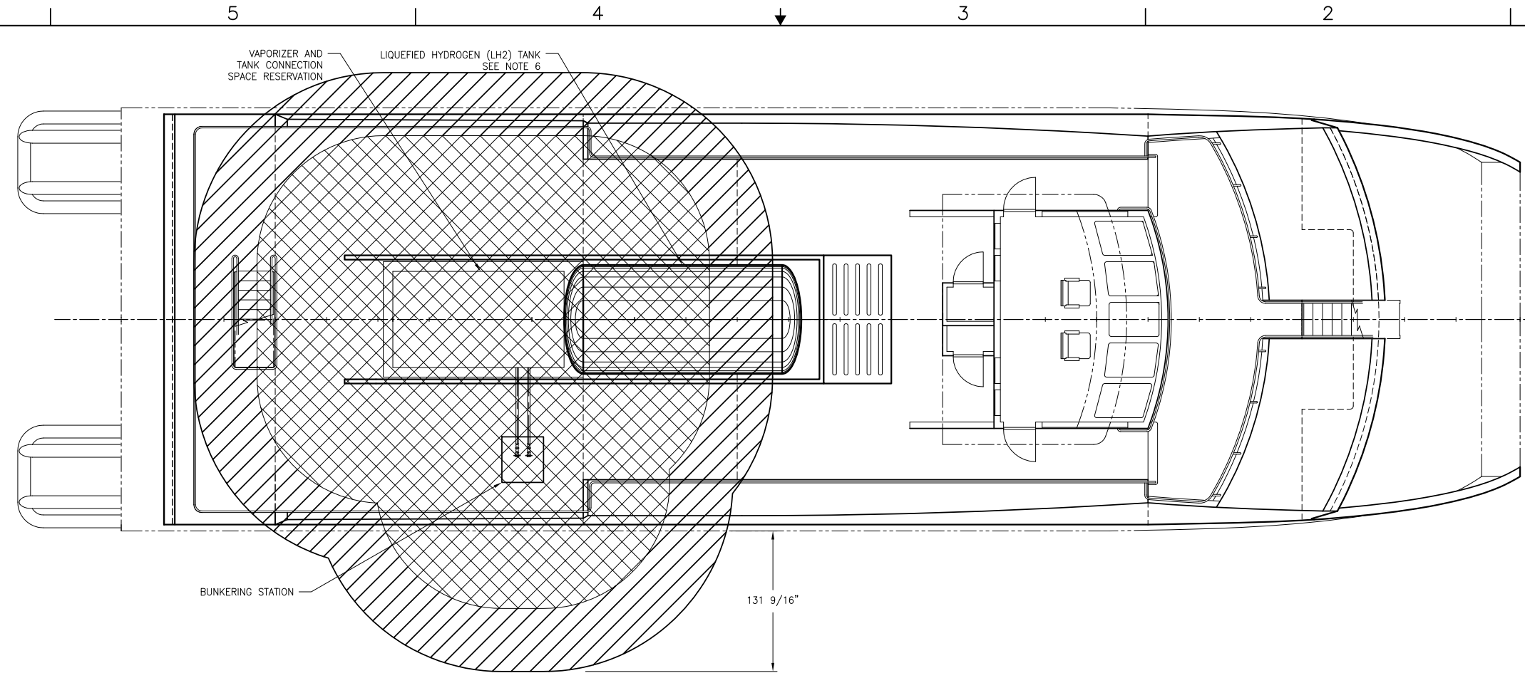
PLAN 3-3C UPPER DECK HAZARDOUS ZONES
