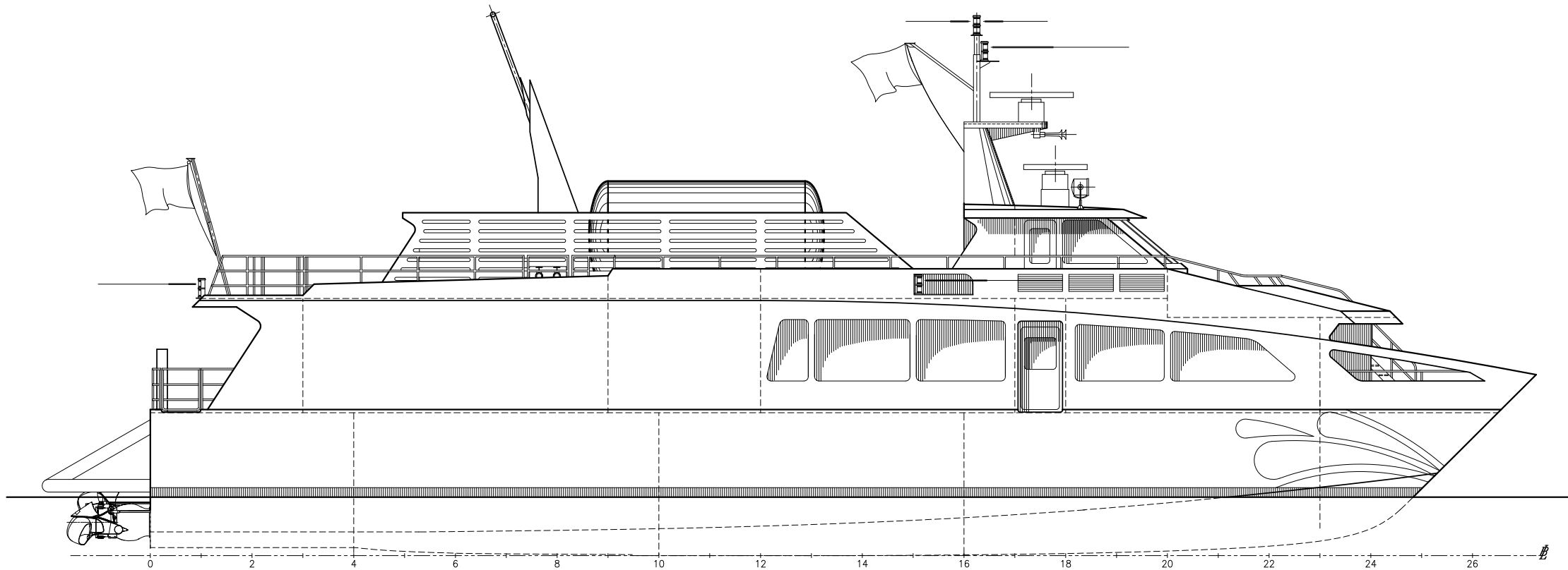
OUTBOARD PROFILE
