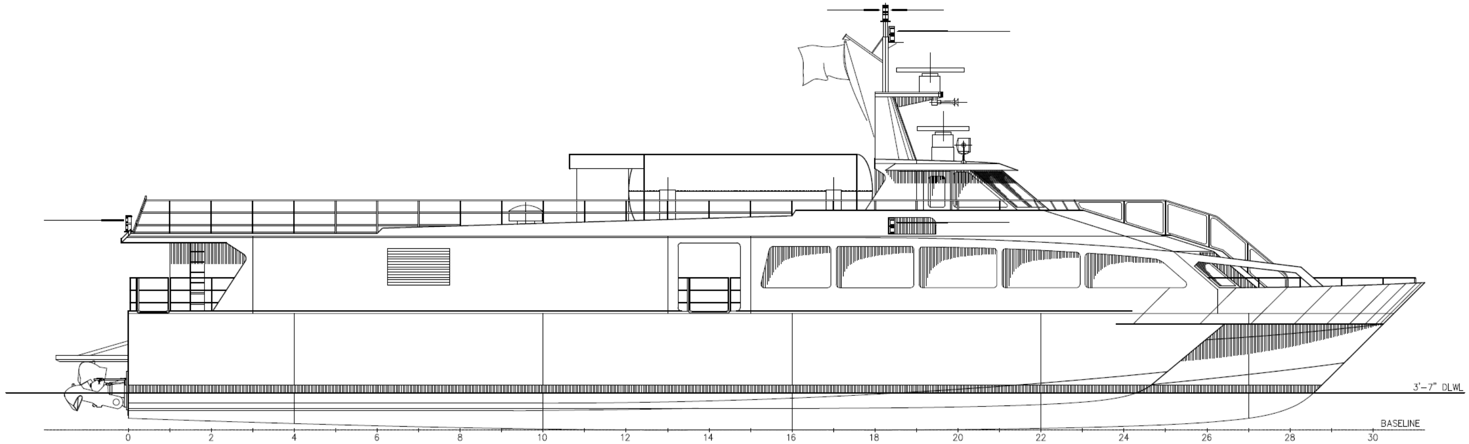
OUTBOARD PROFILE
