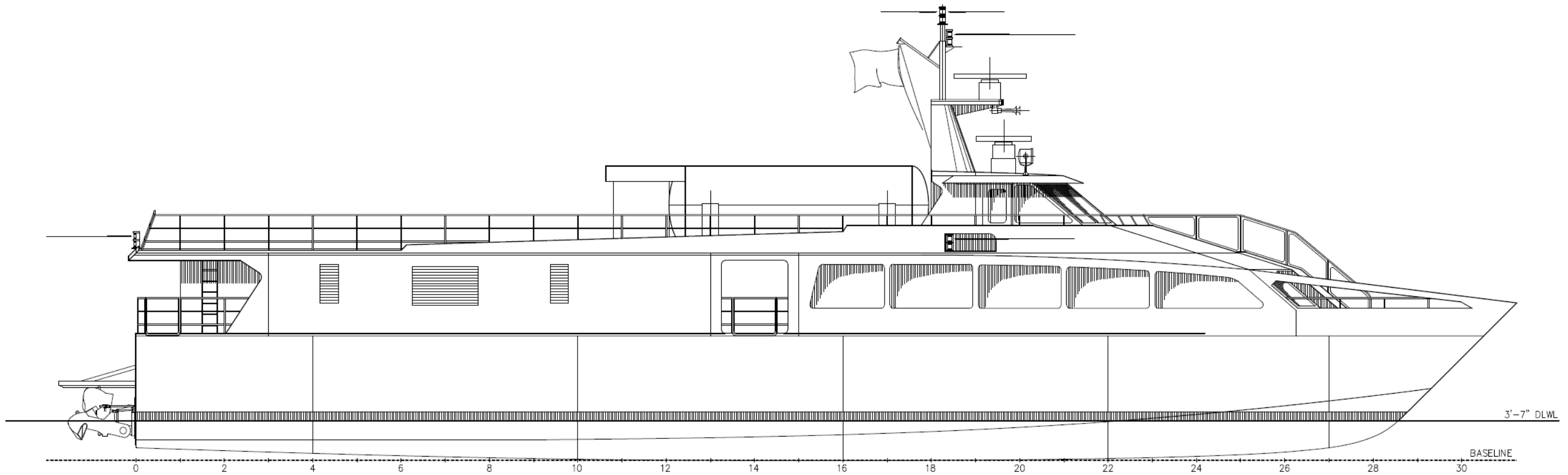
OUTBOARD PROFILE
