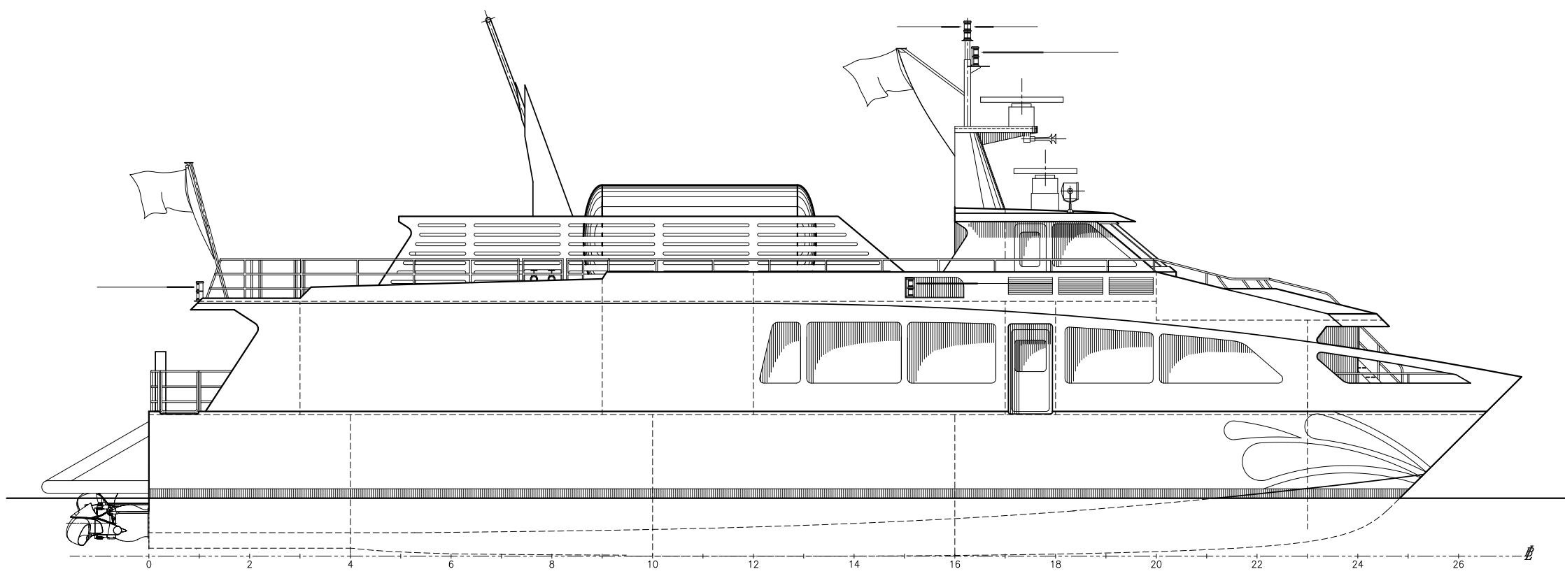
OUTBOARD PROFILE
