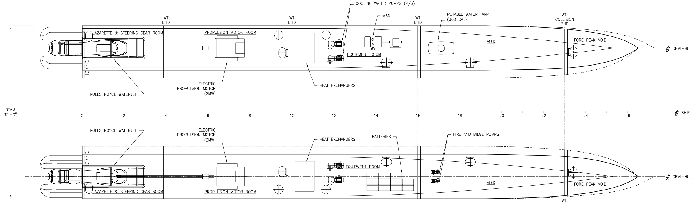
HOLD ARRANGEMENT PLAN
