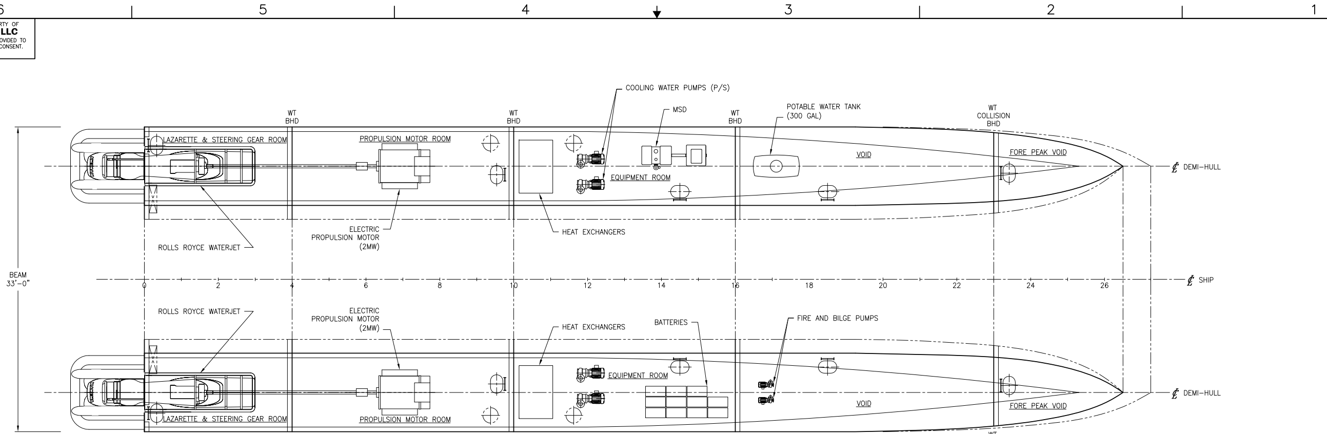
HOLD ARRANGEMENT PLAN
