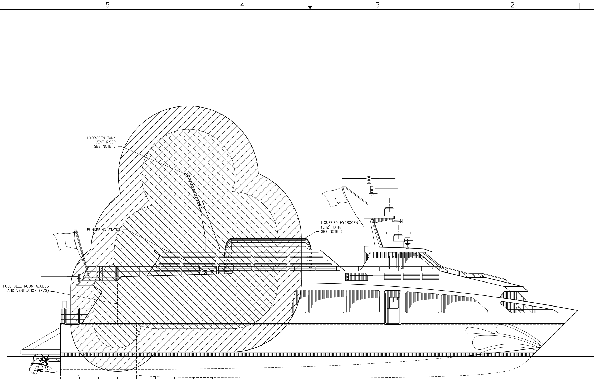
PROFILE 2-3B EXTERIOR HAZARDOUS ZONES NOTE 6
