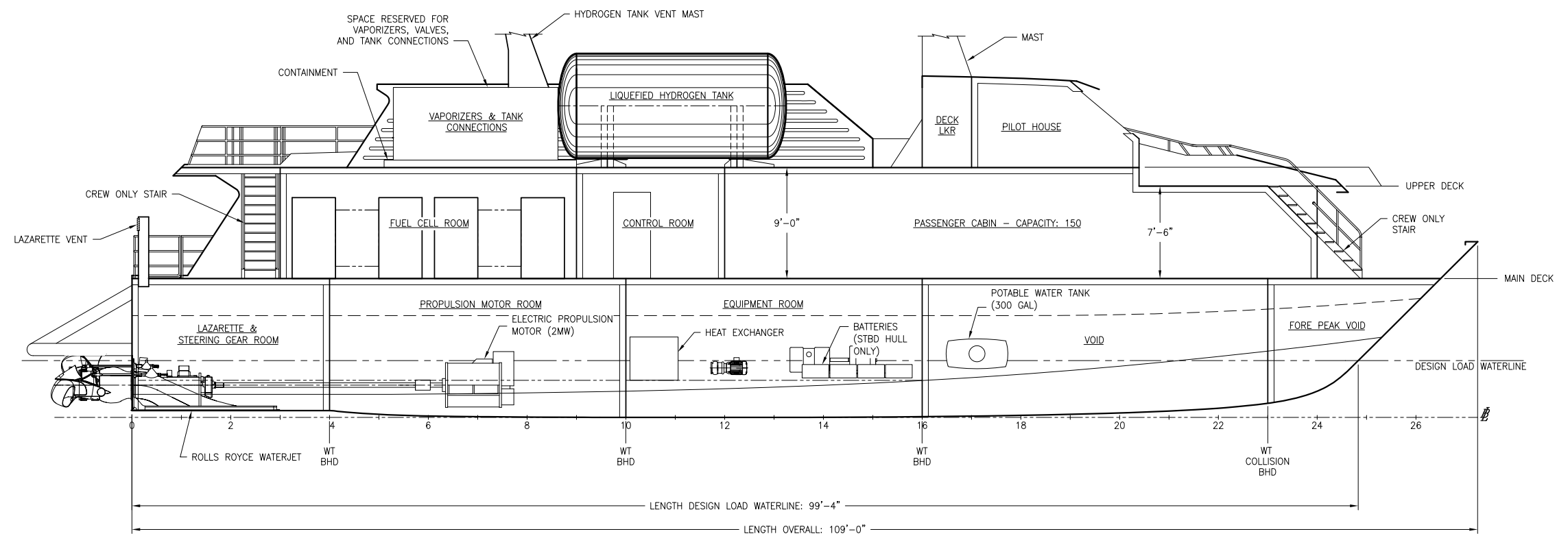
INBOARD PROFILE
