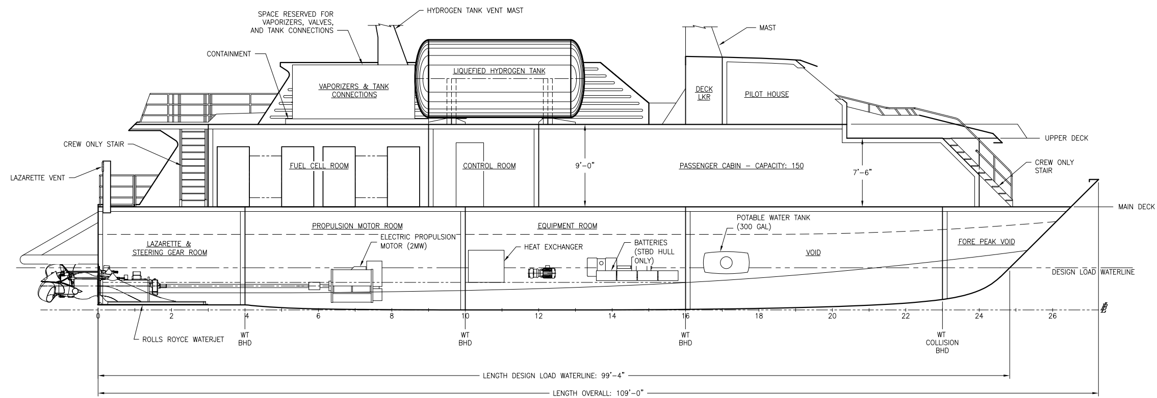
INBOARD PROFILE
